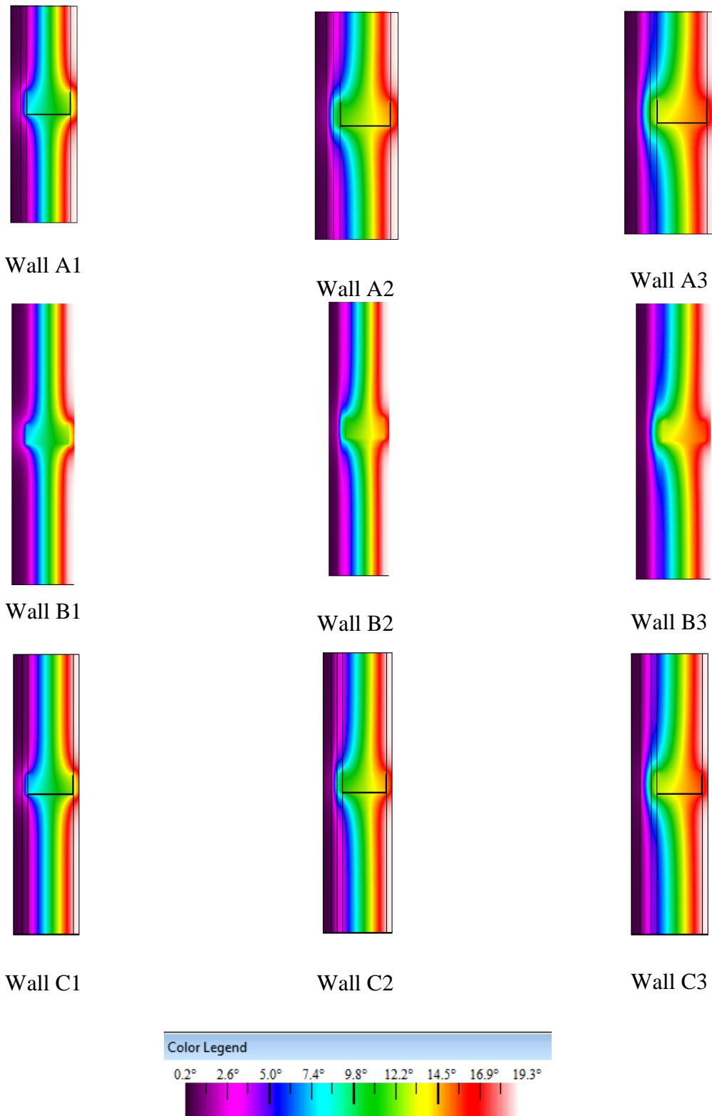
Fig. 2. Temperature profiles
