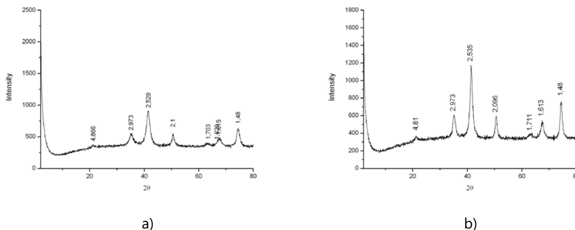
Fig. 1. Diffraction patterns of a synthetic nanomagnetite sample without US treatment (a) and a nanomagnetite sample synthesized under the action of US (b).
